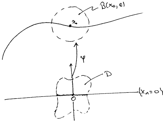
Fig. 22.1. An embedded submanifold of \mathbb{R}^2 .
