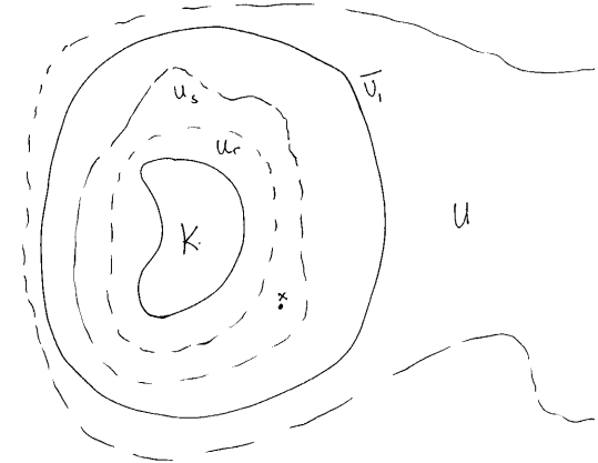
Fig. 3.2. Determining g from \{U_r\} .
