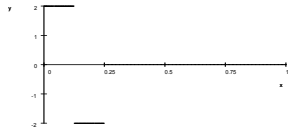
Plot of \psi_{20} .
