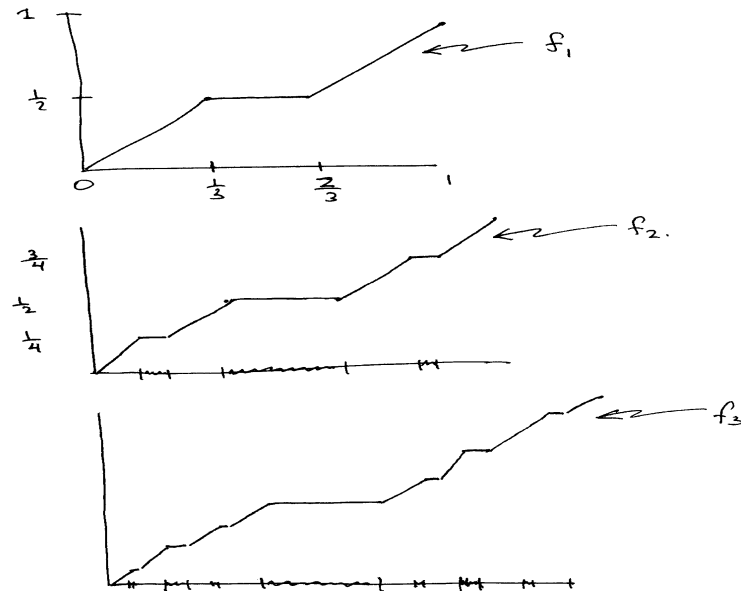
Fig. 20.4. Constructing the Cantor function.
