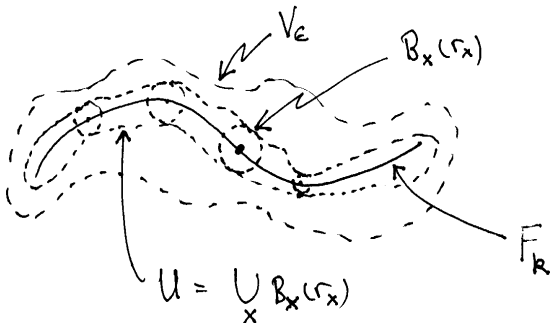
Fig. 20.2. Covering a small set with balls.
