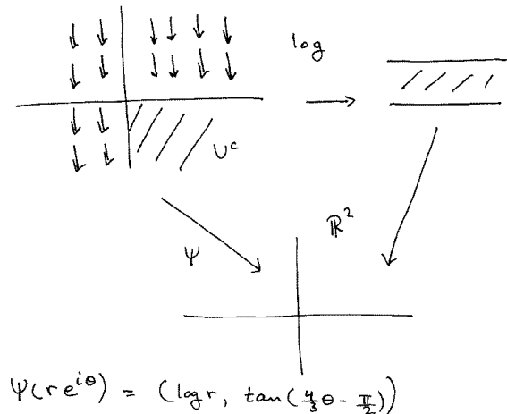
Fig. 6.2. Manufacturing vector fields where b(x) is discontinuous.
