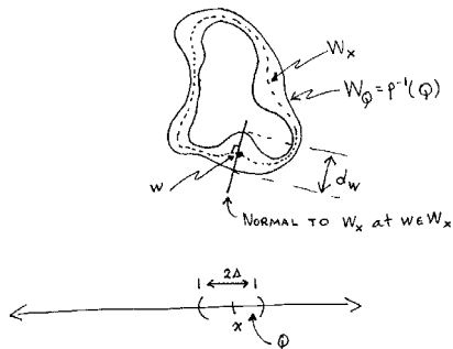
Fig. 25.3. Computing the measure p_*\lambda .
