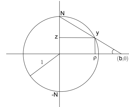
Fig. 3.6. Stereographic projection and the one point compactification of \mathbb{R}^n .
