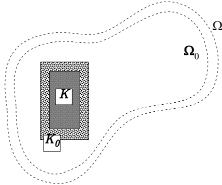
Fig. 29.1. The geometry of K \subset K_0 \subset \Omega_0 \subset \Omega .
