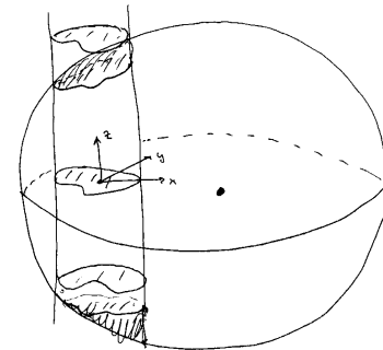
Fig. 34.3. The geometry of the solution to the wave equation in two dimensions.
