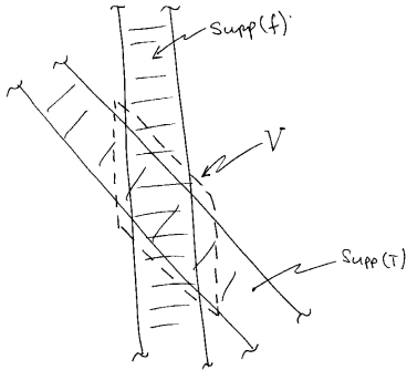
Fig. 34.1. Intersecting the supports.
