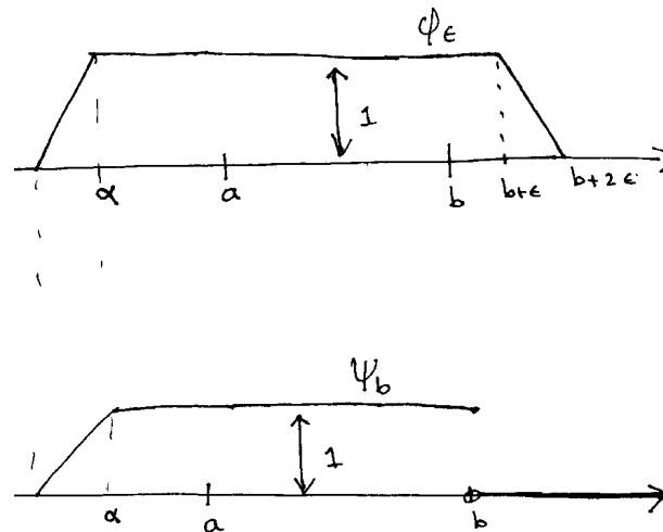
Fig. 20.3. A couple of functions in \overline{\mathcal{S}_c(\mathcal{A})} .
