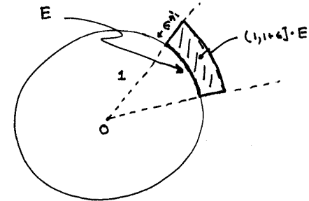
Fig. 9.1. Motivating the definition of surface measure for a sphere.
