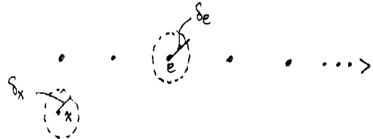
Fig. 2.3. The construction of an open cover with no finite sub-cover.
