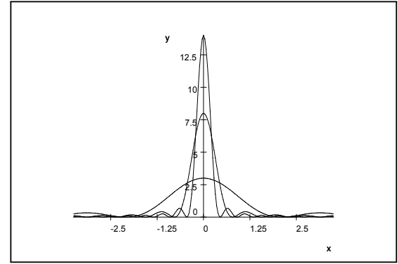
Plots of K_n(\theta) for n = 2, 7 and 13 .
