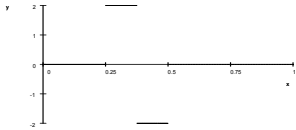
Plot of \psi_{21} .
