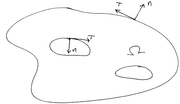
Fig. 22.12. The induced direction for countour integrals along boundaries of regions.
