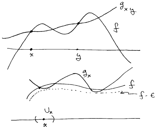
Fig. 11.3. Constructing the functions g_x .
