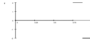
Plot of \psi_{23} .
