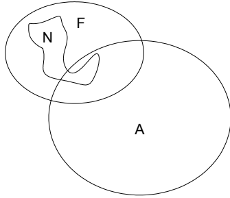
Fig. 8.1. Completing a \sigma -algebra.
