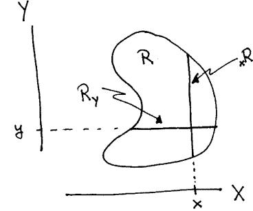
Fig. 1.1. The x and y -slices of a set R \subset X \times Y .
