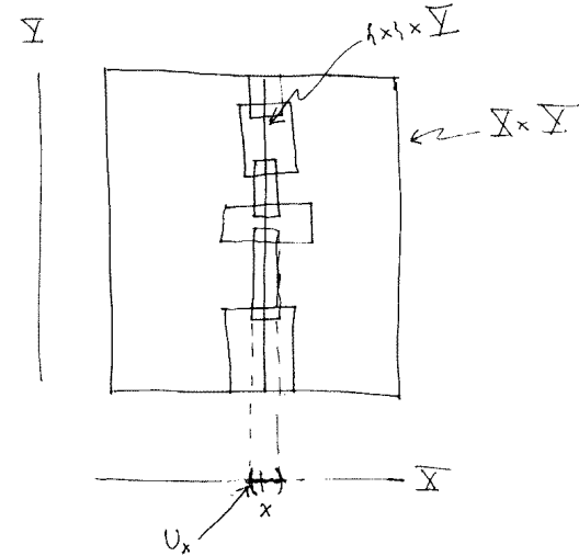
Fig. 27.1. Constructing the open set U_x .
