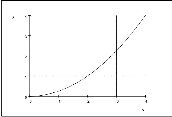
Fig. 1.2. A picture proof of Proposition 1.25.
