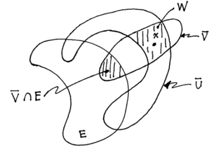
Fig. 3.3. Showing E^c is open.
