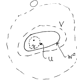
Fig. 3.5. Constructing (U, V) \in \Gamma .
