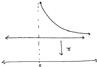
Fig. 25.1. For x > 0 , \pi^{-1}(x) consists of two points while for \pi^{-1}(0) consists of one point for x \leq 0 .
