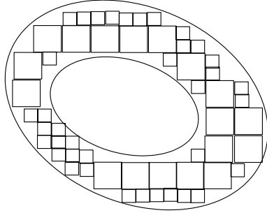
Fig. 21.1. Filling out an open set with half open disjoint cubes. We have drawn \mathcal{F}_2 .
