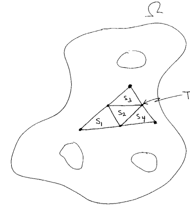
Fig. 30.1. Splitting T into four similar triangles of equal size.
