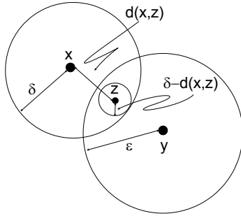
Fig. 7.1. Fitting balls in the intersection.
