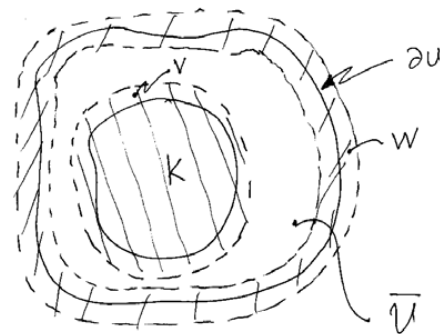
Fig. 3.1. The construction of V .
