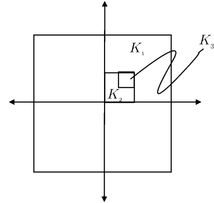
Fig. 2.5. Nested Sequence of cubes.
