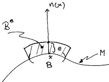
Fig. 22.5. Computing the surface area of B as the volume of an \epsilon -fattened neighborhood of B .
