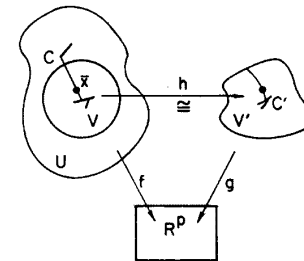
Figure . Construction of the map g
