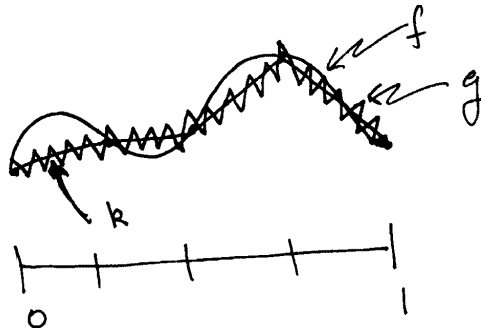
Fig. 27.2. Constructing a rough approximation, g , to a continuous function f .
