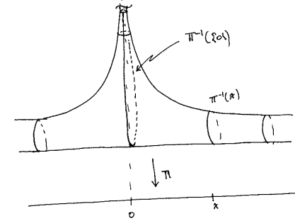
Fig. 25.2. For x \neq 0 , \pi^{-1}(x) is diffeomorphic to a circle while \pi^{-1}(0) is diffeomorphic to a \mathbb{R} .
