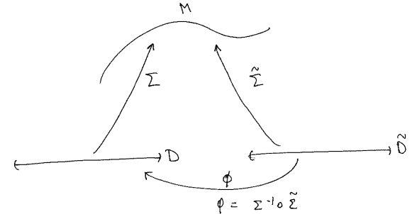
Fig. 22.4. Verifying surface integrals are independent of parametrization.
