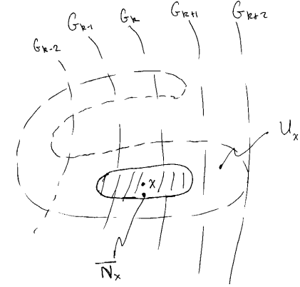
Fig. 3.4. Constructing the \{W_i\}_{i=1}^N .
