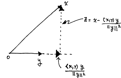
Fig. 14.1. The picture behind the proof.
