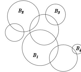
Fig. 20.1. Picking out the large disjoint balls.
