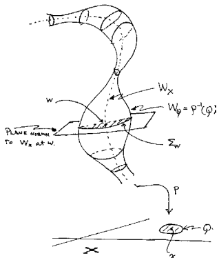
Fig. 25.4. Computing p_*\lambda again.
