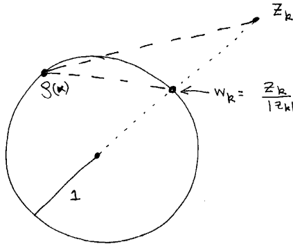
Fig. 18.1. Sliding points to the unit circle.
