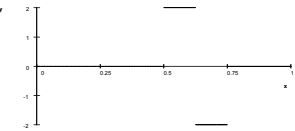
Plot of \psi_{22} .
