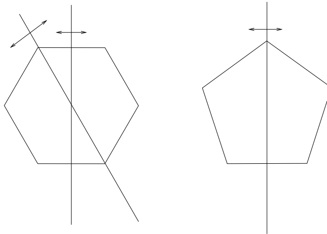
FIGURE 7.1. Conjugacy classes of reflections in dihedral groups
