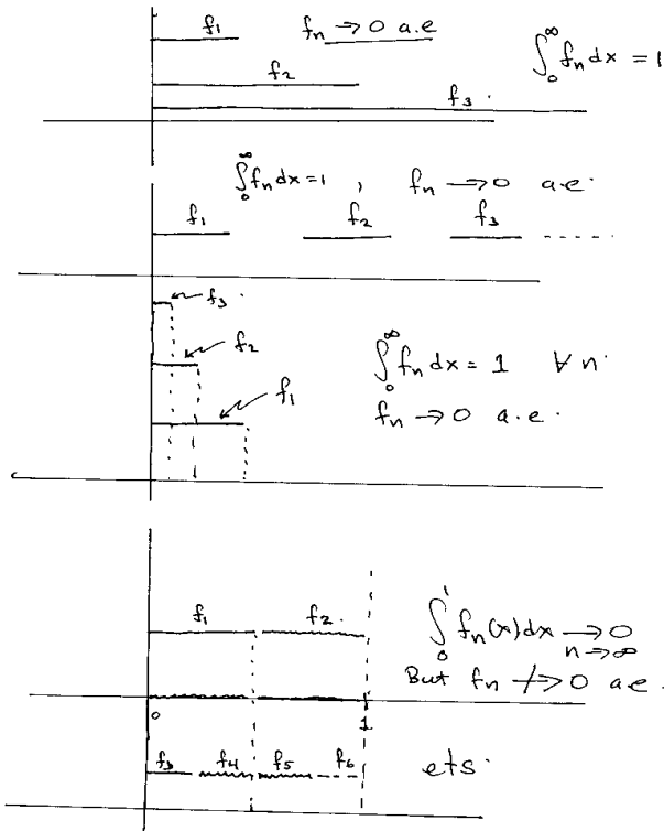
FIGURE 18. Modes of convergence examples. In picture 1. f_n \rightarrow 0 a.e., f_n \not\rightarrow 0 in L^1 , f_n \xrightarrow{m} 0 . In picture 2. f_n \rightarrow 0 a.e., f_n \not\rightarrow 0 in L^1 , f_n \xrightarrow{m} 0 . In picture 3., f_n \rightarrow 0 a.e., f_n \xrightarrow{m} 0 but f_n \not\rightarrow 0 in L^1 . In picture 4., f_n \rightarrow 0 in L^1 , f_n \not\rightarrow 0 a.e., and f_n \xrightarrow{m} 0 .
