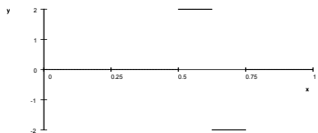
Plot of \psi_22 .
