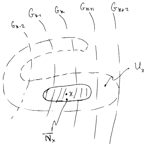
FIGURE 22. Constructing the \{W_i\}_{i=1}^N .
