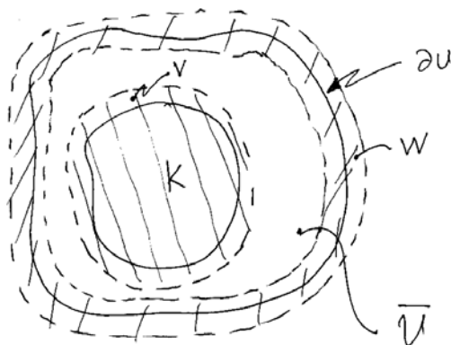
FIGURE 19. The construction of V .
