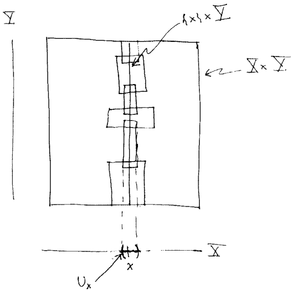
FIGURE 36. Constructing the open set U_x .
