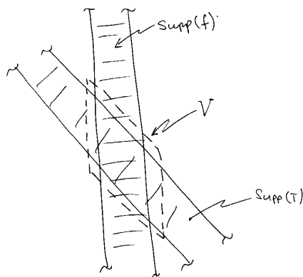
FIGURE 50. Intersecting the supports.
