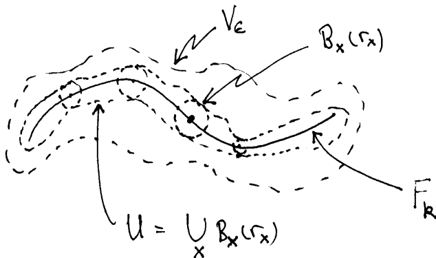
FIGURE 33. Covering a small set with balls.
