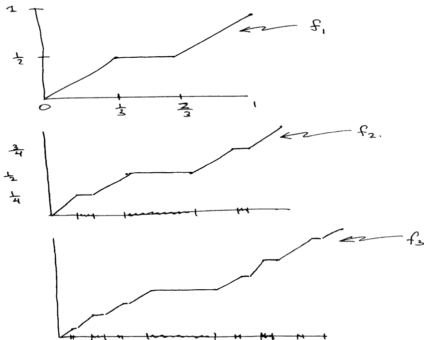
FIGURE 35. Constructing the Cantor function.
