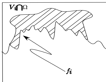
FIGURE 44. The shaded area depicts the support of u_i = \eta_i .
