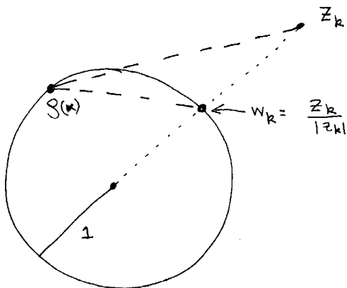
FIGURE 31. Sliding points to the unit circle.
