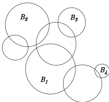
FIGURE 32. Picking out the large disjoint balls.
