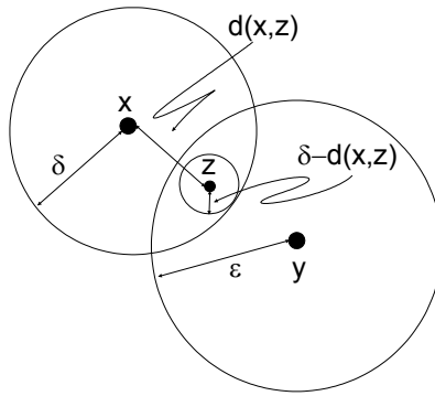
FIGURE 13. Fitting balls in the intersection.
