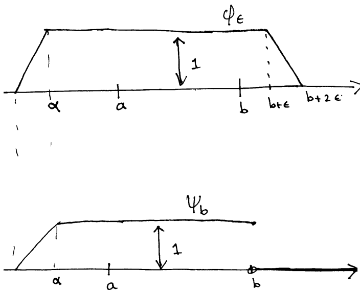
FIGURE 34. A couple of functions in \overline{\mathcal{S}_c(\mathcal{A})} .
