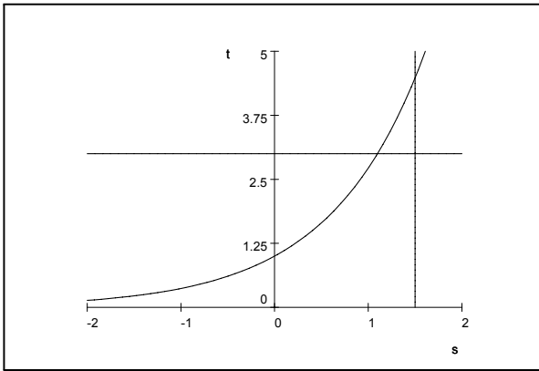
FIGURE 3. Comparing areas when t \geq b goes the same way as in the text.
