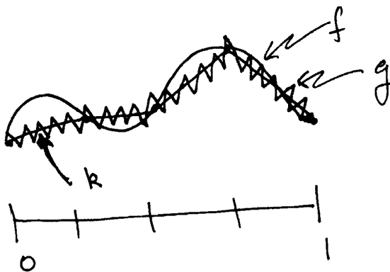
FIGURE 37. Constructing a rough approximation, g , to a continuous function f .
