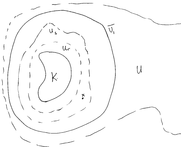
FIGURE 20. Determining g from \{U_r\} .
