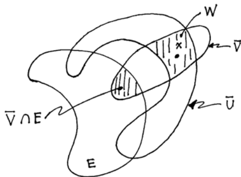
FIGURE 21. Showing E^c is open.
