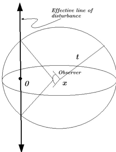
FIGURE 40. The geometry of the solution to the wave equation in two dimensions. A flash at 0 \in \mathbb{R}^2 looks like a line of flashes to the fictitious 3 - d observer and hence she sees the effect of the flash for t \geq |x| . The wave still propagates with speed 1. However there is no longer sharp propagation of the wave front, similar to water waves.
