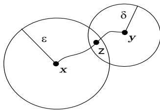
FIGURE 10. An almost length minimizing curve joining x to y .
