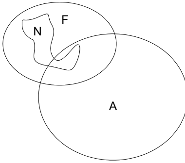
FIGURE 15. Completing a \sigma -algebra.
