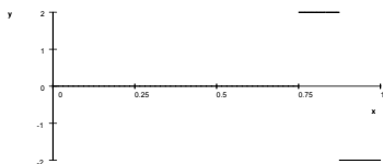
Plot of \psi_23 .
