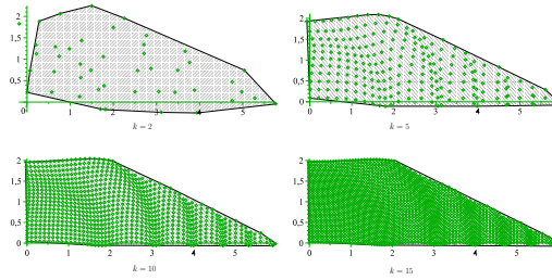
FIGURE 3. Convergence of convex hulls of spectra
