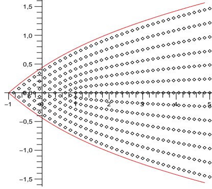
FIGURE 2. Joint spectrum of quantum Jaynes-Cummings model .
