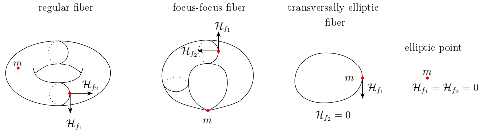
FIGURE 1. Some possible singularities of an integrable system.
