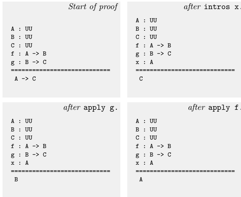
FIGURE 6. Coq output during indirect definition of function composition.
