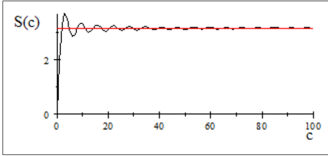
Fig. 28.1. The graph of S(c) in black and \pi in red.
