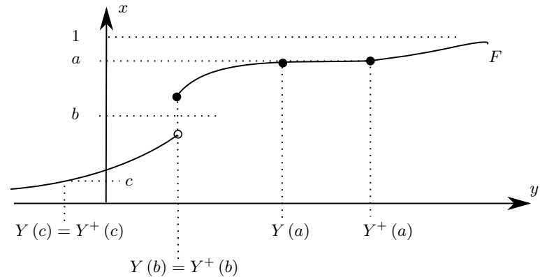
Fig. 27.2. The functions Y and Y^+ associated to F .
