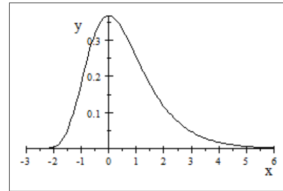
Fig. 27.4. Here is a plot of the density function for Y when \lambda = 1 .
