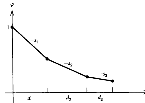
Fig. 28.3. Here is a piecewise linear convex function. We will assume that d_n > 0 for all n and that \varphi(\lambda) = 0 for \lambda sufficiently large. This last restriction may be removed later by a limiting argument.
