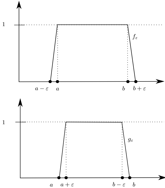
Fig. 27.3. The picture definition of the trapezoidal functions, f_\varepsilon and g_\varepsilon .
