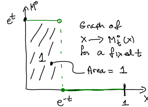
Fig. 34.1. The graph of x \rightarrow M_t^0(x) for some fixed t .
