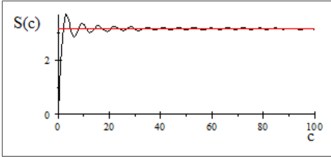
Fig. 29.1. The graph of S(c) in black and \pi in red.
