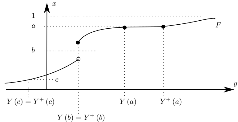
Fig. 28.2. The functions Y and Y^+ associated to F .
