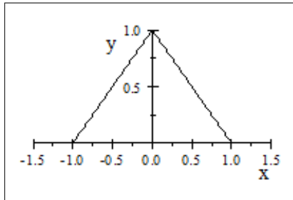
Fig. 29.2. The triangular density function.
