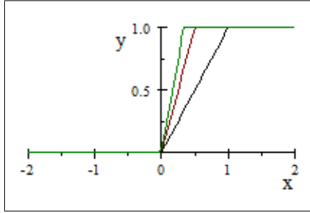
Fig. 12.1. Plots of \varphi_1, \varphi_2 and \varphi_3 which are continuous functions used to approximate, x \rightarrow 1_{x \geq 0} .
