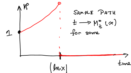
Fig. 35.2. A typical sample path of M_t^0(x) .
