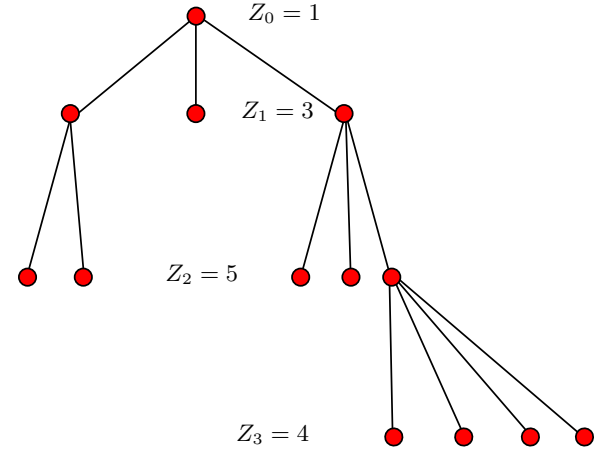
Fig. 24.1. A possible realization of a Galton Watson “tree.”
