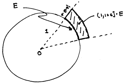
Fig. 13.5. Motivating the definition of surface measure for a sphere.
