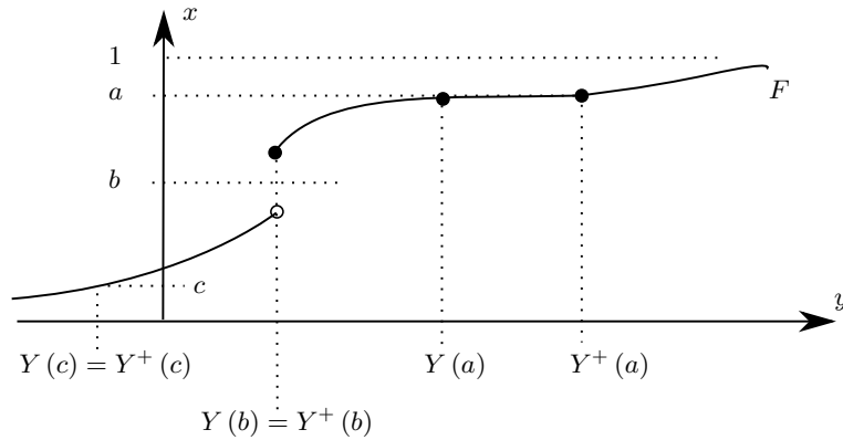
Fig. 25.3. The functions Y and Y^+ associated to F .
