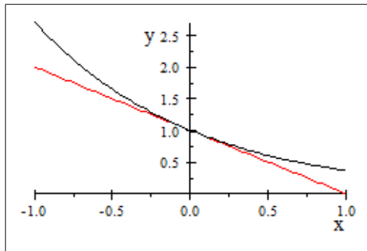
Fig. 14.1. A graph of 1 - x and e^{-x} showing that 1 - x \leq e^{-x} for all x .
