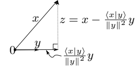
Fig. 17.1. The picture behind the proof of the Schwarz inequality.
