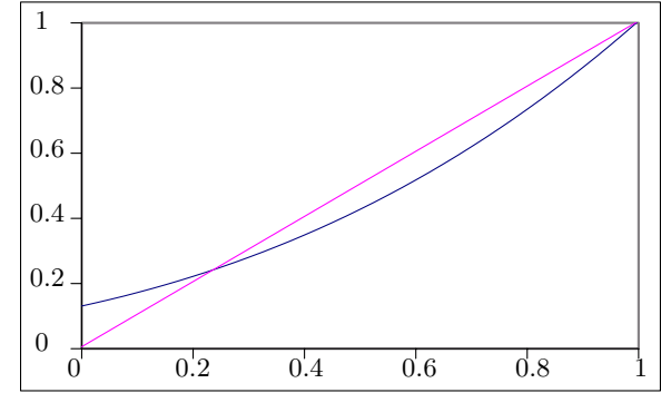
Fig. 23.2. Figure associated to \varphi(s) = \frac{1}{8}(1 + 3s + 3s^2 + s^3) which is relevant for Exercise 3.13 of Durrett on p. 249. In this case \rho \cong 0.23607 .
