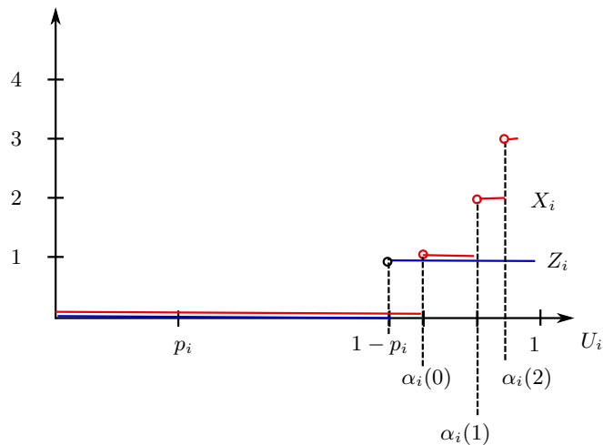
Fig. 25.1. Plots of X_i and Z_i as functions of U_i .
