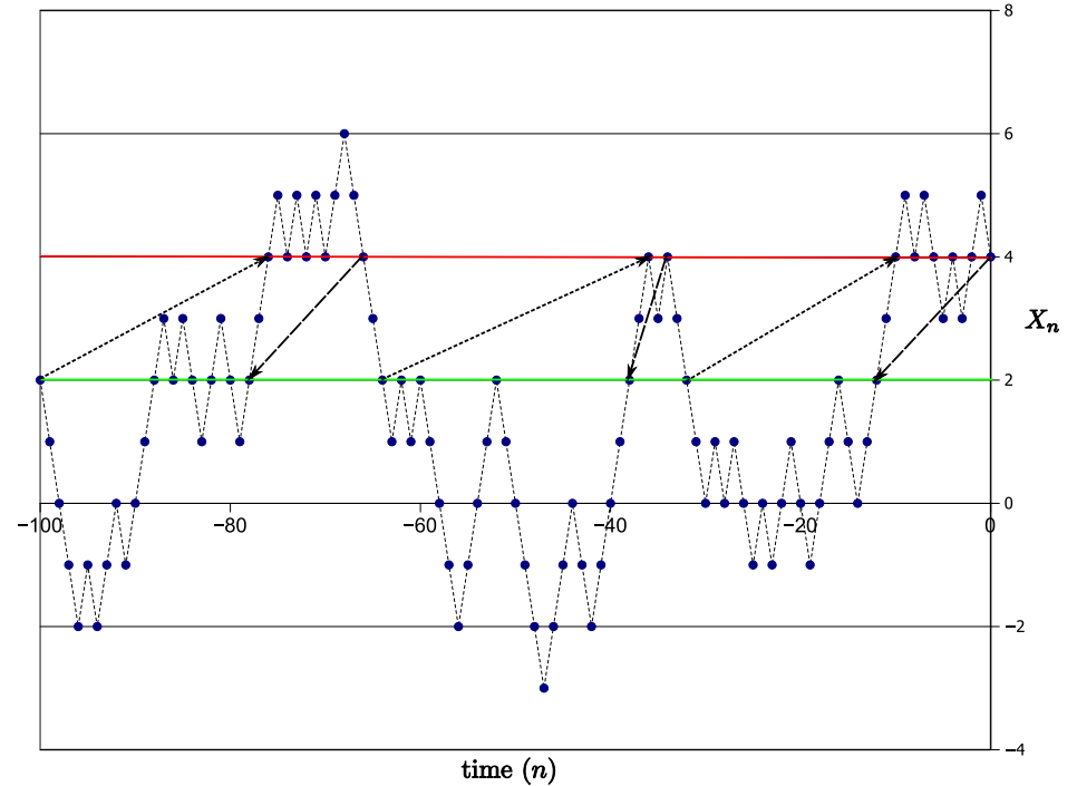
Fig. 22.5. A sample path of a backwards martingale on [-100, 0] indicating the down crossings of X_0, X_{-1}, \dots, X_{-100} and the upcrossings of X_{-100}, X_{-99}, \dots, X_0 . The total number of each is the same.
