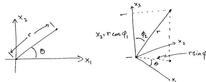
Fig. 13.6. Setting up polar coordinates in two and three dimensions.
