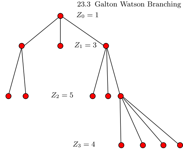
Fig. 23.1. A possible realization of a Galton Watson “tree.”
