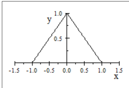
Fig. 26.2. The triangular density function.
