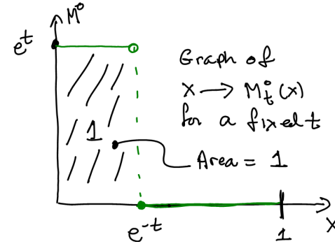
Fig. 32.1. The graph of x \rightarrow M_t^0(x) for some fixed t .
