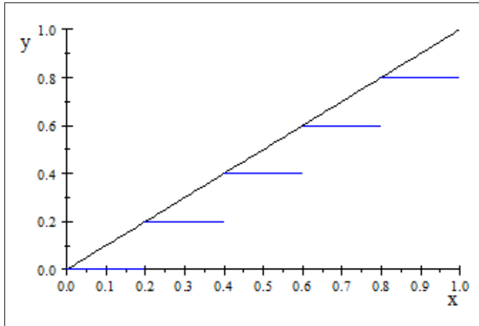
Fig. 25.2. The plot of F_5 in blue and F is black on [0, 1] .
