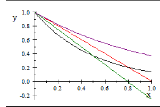
Fig. 14.2. A graph of 1 - x (in red), the line joining (0, 1) and (1/2, e^{-1}) (in green), e^{-x} (in purple), and e^{-2x} (in black) showing that e^{-2x} \leq 1 - x \leq e^{-x} for all x \in [0, 1/2] .
