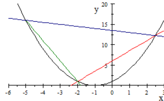
Fig. 16.3. A convex function along with three chords corresponding to x_0 = -5 and x_1 = -2 , x_0 = -2 and x_1 = 5/2 , and x_0 = -5 and x_1 = 5/2 with slopes, m_1 = -15/3 , m_2 = 15/6 and m_3 = -1/2 respectively. Notice that m_1 \leq m_3 \leq m_2 .
