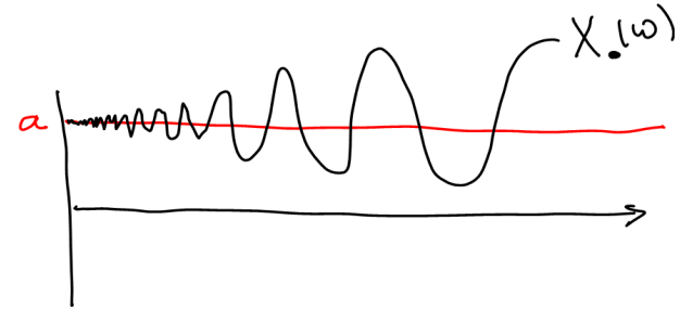
Fig. 31.1. A sample point, \omega \in \Omega , where T_A(\omega) = 0 with A = \{a\} \subset \mathbb{R} .
