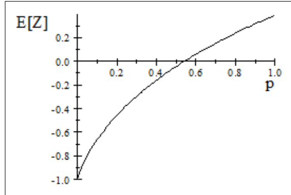
Fig. 22.1. The graph of \mathbb{E}[\ln(p+U)] as a function of p . This function has a zero at p = p_c \cong 0.54221 .
