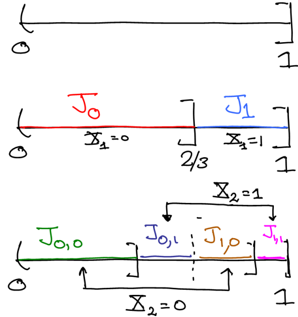
Fig. 14.3. Here we suppose that p_0 = 2/3 and p_1 = 1/3 and then we construct J_i and J_{i,k} for l, k \in \{0, 1\} .
