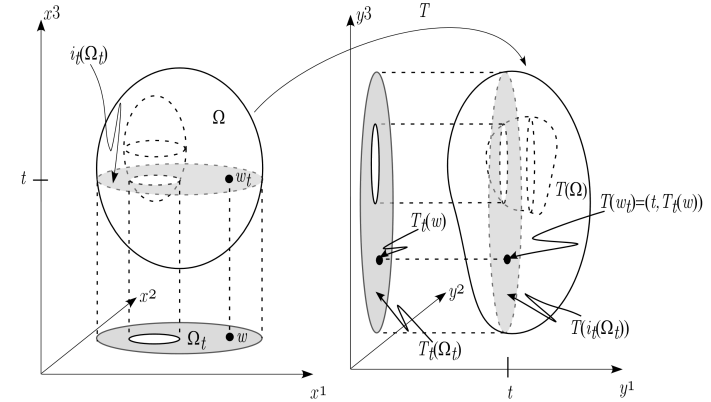
Fig. 13.2. In this picture d = i = 3 and \Omega is an egg-shaped region with an egg-shaped hole. The picture indicates the geometry associated with the map T and slicing the set \Omega along planes where x_3 = t .
