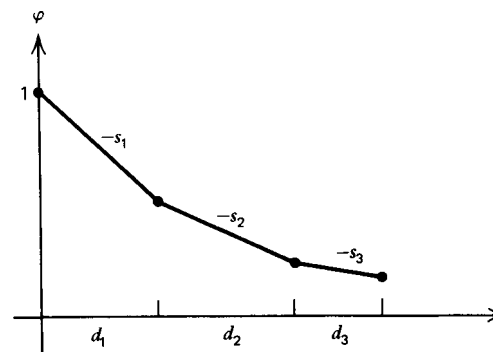
Fig. 26.3. Here is a piecewise linear convex function. We will assume that d_n > 0 for all n and that \varphi(\lambda) = 0 for \lambda sufficiently large. This last restriction may be removed later by a limiting argument.
