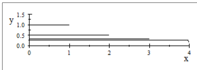
Fig. 16.1. Graphs of f_n = \frac{1}{n}1_{[0,n]} for n = 1, 2, 3, 4 .
