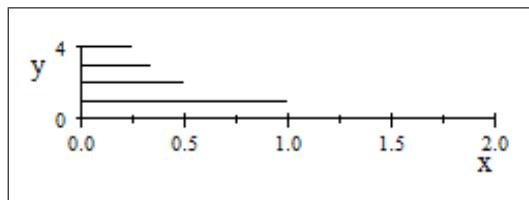
Fig. 16.2. Graphs of f_n = n \cdot 1_{[0,1/n]} for n = 1, 2, 3, 4 .
