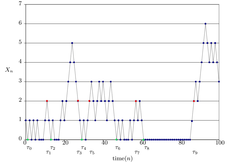
Fig. 22.4. A sample path of a positive submartingale along with stopping times \tau_{2j} and \tau_{2j+1} which are the successive hitting times of 0 and 2 respectively. If we take N = 70 in this case, then observe that X_{\tau_7 \wedge 70} - X_{\tau_6 \wedge 70} \geq 2 while X_{\tau_9 \wedge 70} - X_{\tau_8 \wedge 70} = 0 .
