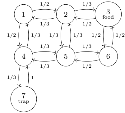
Fig. 21.3. The jump diagram for our proverbial rat in the maze.
