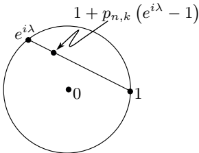
Fig. 27.1. Simple circle geometry reflecting the convexity of the disk.
