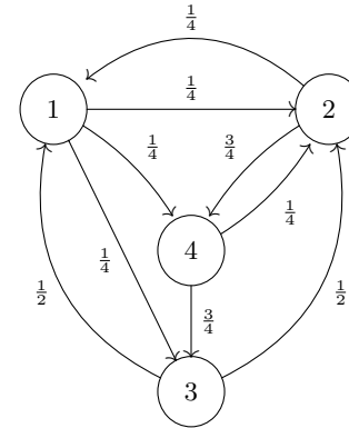
Fig. 21.8. The jump diagram for Q .
