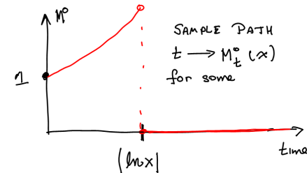
Fig. 32.2. A typical sample path of M_t^0(x) .
