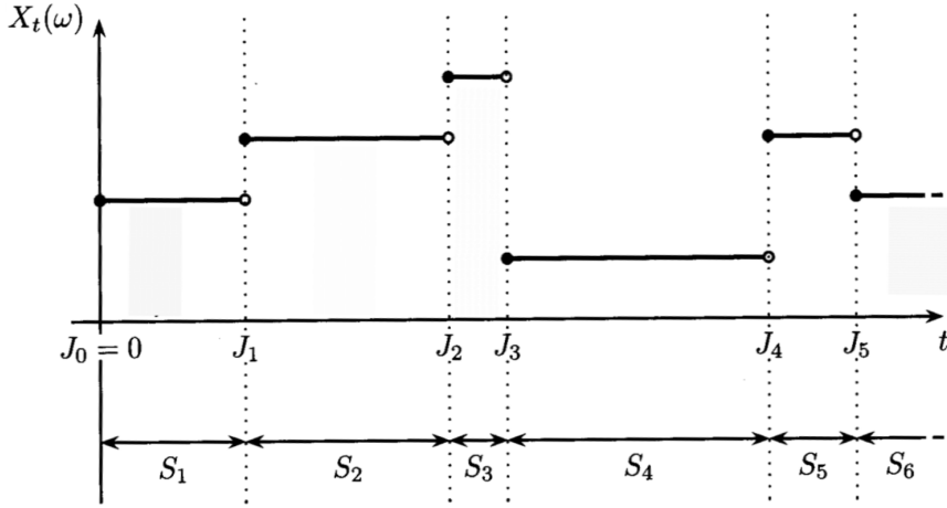
Fig. 21.2. Typical sample paths of a continuous time Markov chain in a discrete state space.
