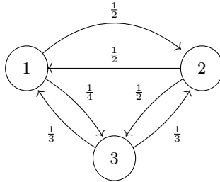
Fig. 21.7. In the above diagram there are jumps from 1 to 1 with probability 1/4 and jumps from 3 to 3 with probability 1/3 which are not explicitly shown but must be inferred by conservation of probability.
