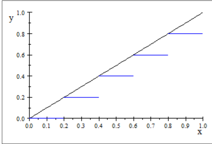
Fig. 26.2. The plot of F_5 in blue and F is black on [0, 1] .
