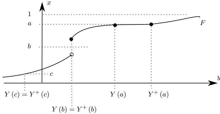
Fig. 26.3. The functions Y and Y^+ associated to F .
