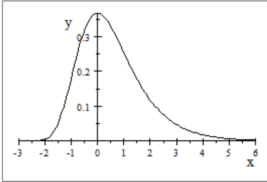
Fig. 26.5. Here is a plot of the density function for Y when \lambda = 1 .
