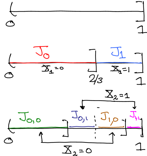
Fig. 15.4. Here we suppose that p_0 = 2/3 and p_1 = 1/3 and then we construct J_l and J_{l,k} for l, k \in \{0, 1\} .
