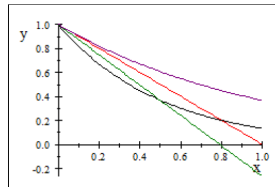
Fig. 15.3. A graph of 1 - x (in red), the line joining (0, 1) and (1/2, e^{-1}) (in green), e^{-x} (in purple), and e^{-2x} (in black) showing that e^{-2x} \leq 1 - x \leq e^{-x} for all x \in [0, 1/2] .
