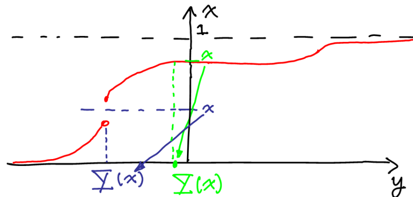
Fig. 9.3. A pictorial definition of Y(x) .
