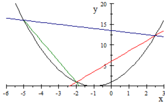
Fig. 17.3. A convex function along with three cords corresponding to x_0 = -5 and x_1 = -2 , x_0 = -2 and x_1 = 5/2 , and x_0 = -5 and x_1 = 5/2 with slopes, m_1 = -15/3 , m_2 = 15/6 and m_3 = -1/2 respectively. Notice that m_1 \leq m_3 \leq m_2 .
