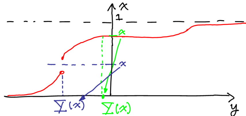
Fig. 9.3. A pictorial definition of Y(x) .
