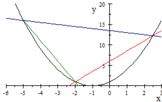
Fig. 17.3. A convex function along with three cords corresponding to x_0 = -5 and x_1 = 5/2 , x_0 = -5 and x_1 = 5/2 with slopes, m_1 = -15/3 , m_2 = 15/6 and m_3 = -1/2 respectively. Notice that m_1 \leq m_3 \leq m_2 .
