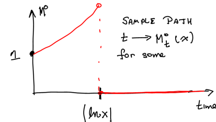
Fig. 33.2. A typical sample path of M^0(x) .
