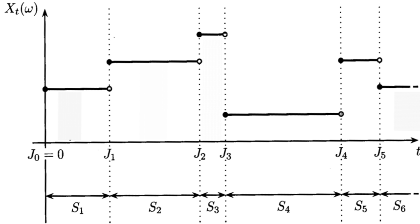
Fig. 19.2. Typical sample paths of a continuous time Markov chain in a discrete state space.
