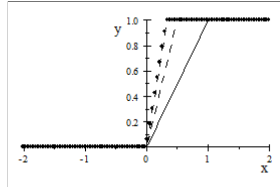
Fig. 10.1. Plots of \varphi_1 , \varphi_2 and \varphi_3 .
