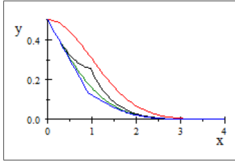
Fig. 9.1. Plots of P(X \geq x) and its estimates.
