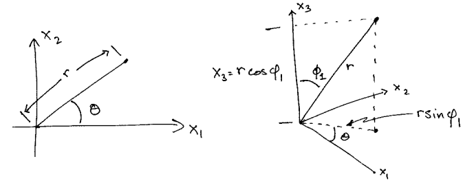
Fig. 11.6. Setting up polar coordinates in two and three dimensions.
