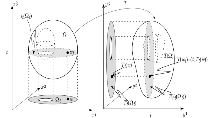
Fig. 11.2. In this picture d = i = 3 and \Omega is an egg-shaped region with an egg-shaped hole. The picture indicates the geometry associated with the map T and slicing the set \Omega along planes where x_3 = t .
