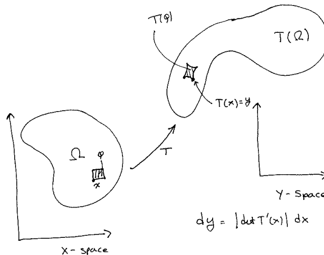
Fig. 11.1. The geometric setup of Theorem 11.21.
