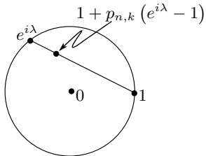
Fig. 25.1. Simple circle geometry reflecting the convexity of the disk.
