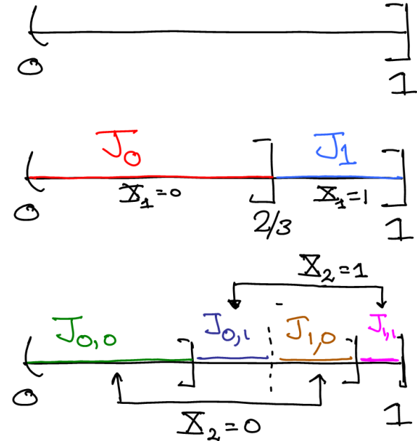
Fig. 12.3. Here we suppose that p_0 = 2/3 and p_1 = 1/3 and then we construct J_l and J_{l,k} for l, k \in \{0, 1\} .
