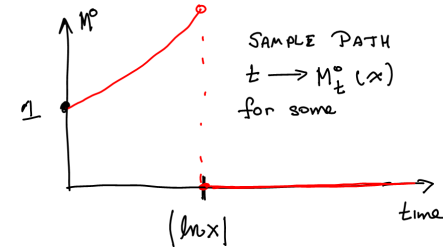
Fig. 30.2. A typical sample path of M^0(x) .
