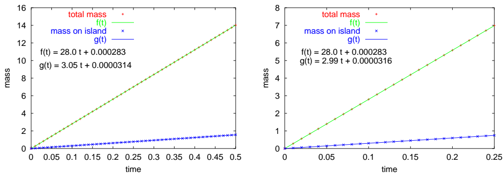
Figure 10: Mass increase: circular island (left) and perturbed circular island (right).
