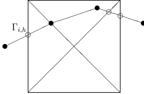
Figure 6: Element T , boundary \Gamma_{i,h} , and line integration path.
