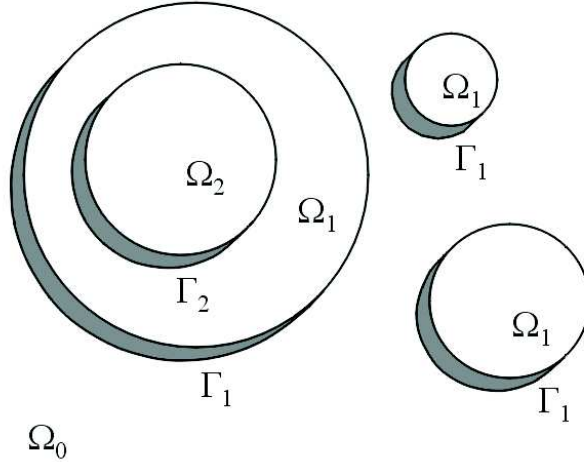
Figure 2: Schematic description of terraces \Omega_i = \Omega_i(t) and boundaries \Gamma_i = \Gamma_i(t) .
