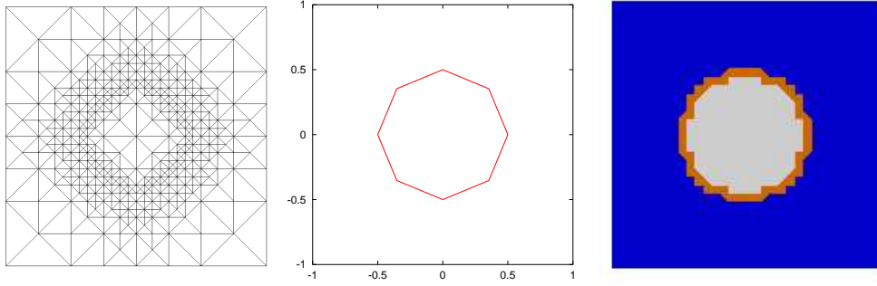
Figure 4: A refined 2d mesh, a 1d mesh of a boundary, and element marking.
