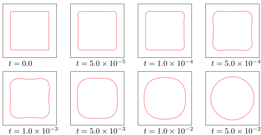
Case 3: mean curvature and surface diffusion
