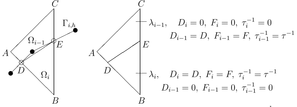
Figure 5: Element T , boundary \Gamma_{i,h} , and definition of \lambda , D_i , F_i , and \tau_i^{-1} .
