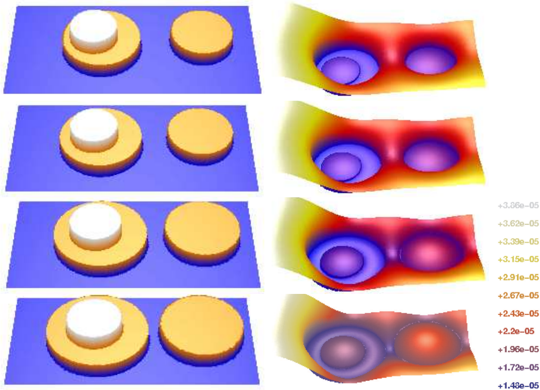
Figure 14: Discrete height function and adatom density at various times.
