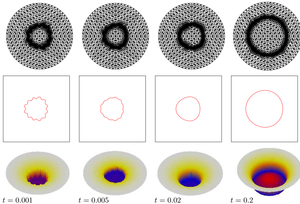
Figure 13: 2d mesh, 1d boundary and adatom density: without surface diffusion.
