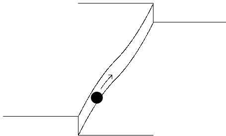
Figure 1: One-dimensional “surface” diffusion.
