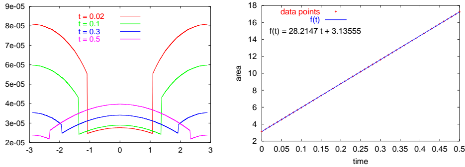
Figure 11: Adatom density profile (left) and area growth rate (right).
