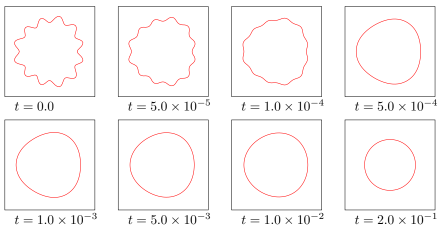
Case 3: mean curvature and surface diffusion
