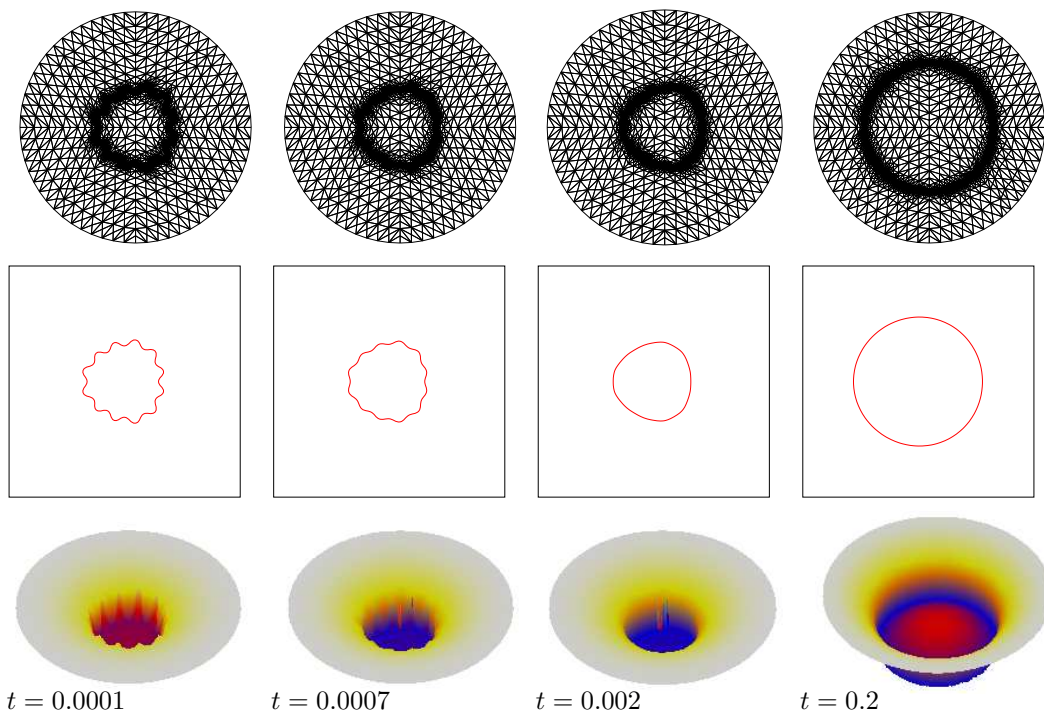
Figure 12: 2d mesh, 1d boundary and adatom density: with surface diffusion.
