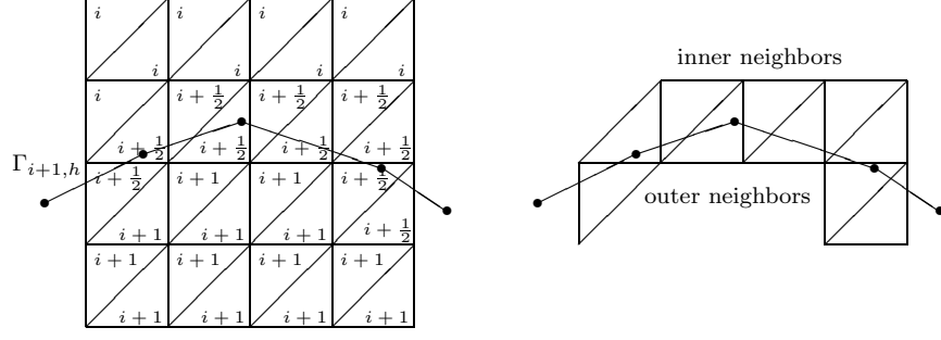
Figure 3: Marking of elements T in a triangulation \mathcal{T}_h near a boundary \Gamma_{i+1,h} .
