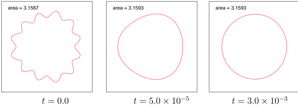
Figure 9: Conservation of the island area in the case k_+ = k_- = 0 .
