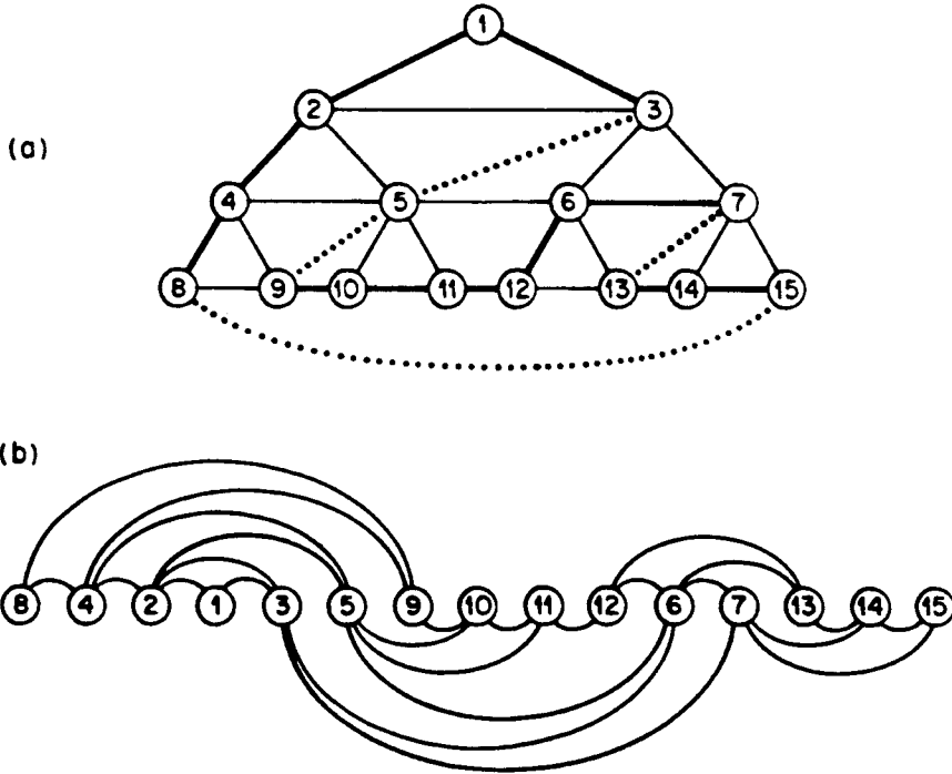
FIG. 4. (a) An edge-augmentation of the depth-4 X -tree and an efficient hamiltonian cycle. (b) The layout of the X -tree induced by the cycle of (a).
