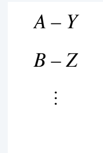
Gale-Shapley matching S^*
