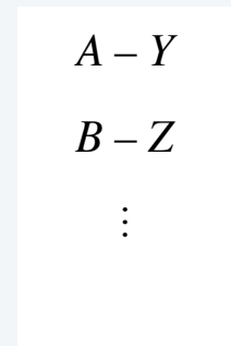
stable matching S
