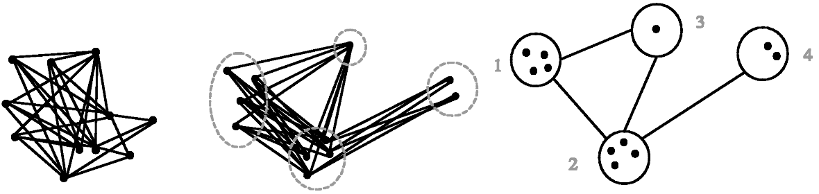
FIG. 2. A graph, shown on the left , can be described as a set of orbits ( middle diagram) connected as shown on the right . Matrix \mathbf{C} is the adjacency matrix of the right graph, and \mathbf{v} is the vector of the occupation numbers. The rightmost panel shows how the vertices can be grouped into the four orbits of the graph; thus, the \mathbf{v} vector is simply (4, 4, 1, 2).
