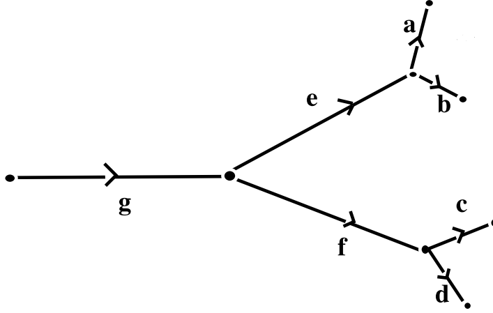
Figure 6: \Gamma_2
