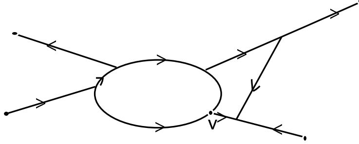
Figure 1: An object \Gamma in \mathcal{C}_{2,2+2}
