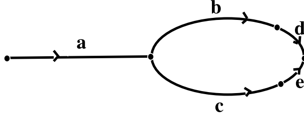
Figure 9: \Gamma_4
