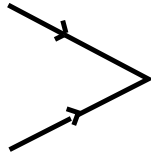
Figure 10: \Gamma_0
