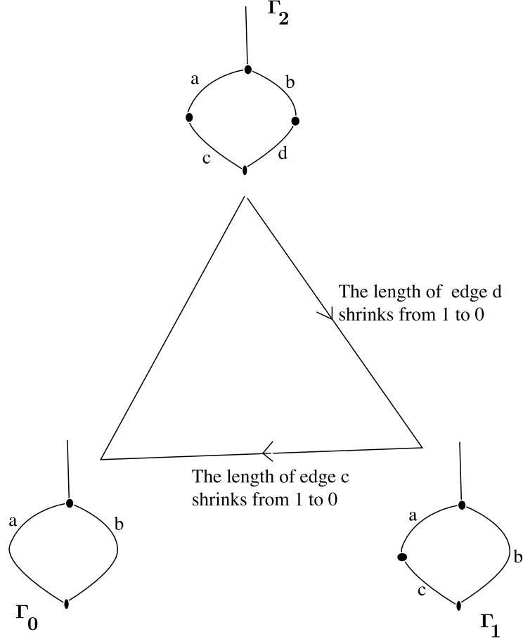
Figure 3: A 2-simplex of metrics.
