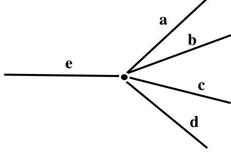
Figure 8: \Gamma_3
