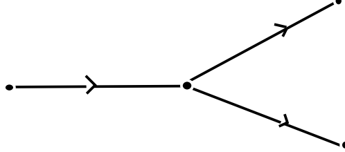
Figure 5: \Gamma_1
