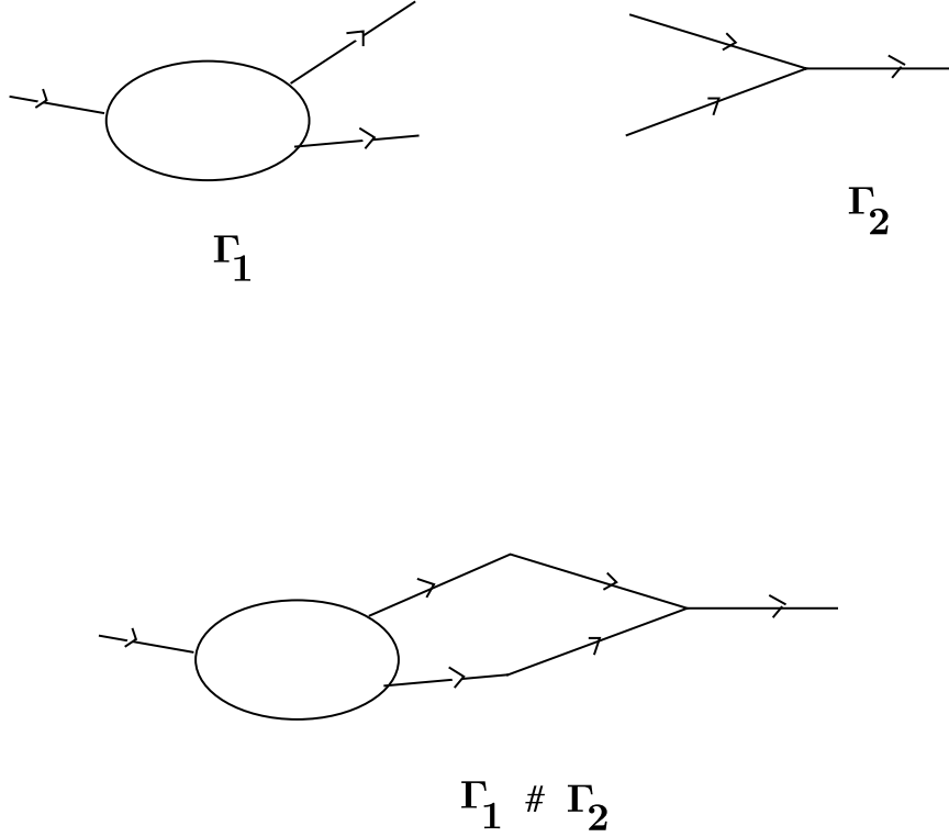
Figure 4: \Gamma_1 \# \Gamma_2
