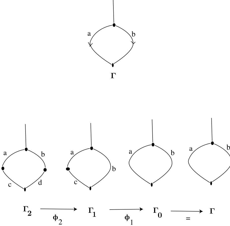
Figure 2: A 2-simplex in |\mathcal{C}_\Gamma| .
