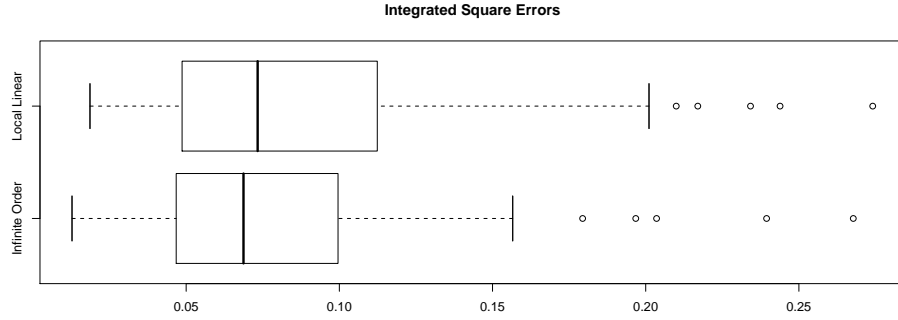
Figure 4: Comparison of integrated square errors for 100 simulations of the exponential function with n = 200 and \sigma = 0.5 .
