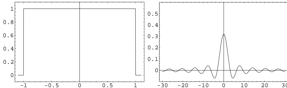
Figure 1: \lambda(s) and the resulting Dirichlet kernel.
