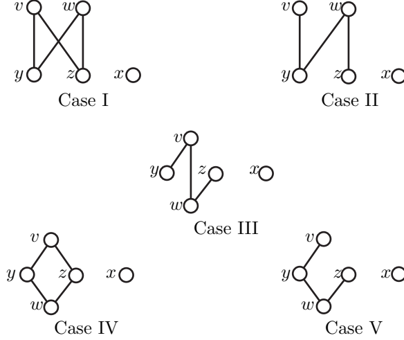
FIGURE 6. The five cases for Lemma 8
