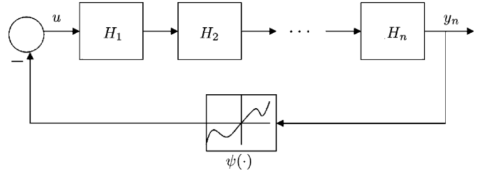
Fig. 2. The feedback interconnection for Corollary 2.
