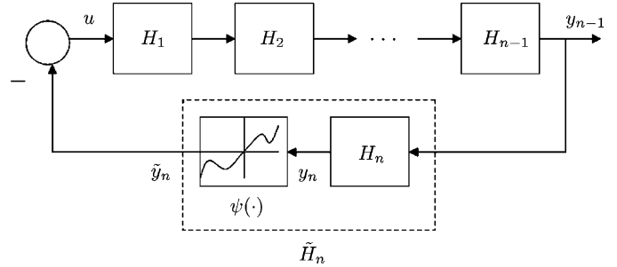
Fig. 3. An equivalent representation of the feedback system in Fig. 2. When H_n is a linear block H_n(s) = \beta_n/(s + \alpha_n) , its series interconnection with the [0, \kappa] sector nonlinearity \psi(\cdot) constitutes a dynamic block \tilde{H}_n which satisfies the OSP property (15) with \tilde{\gamma}_n = \kappa(\beta_n/\alpha_n) .
